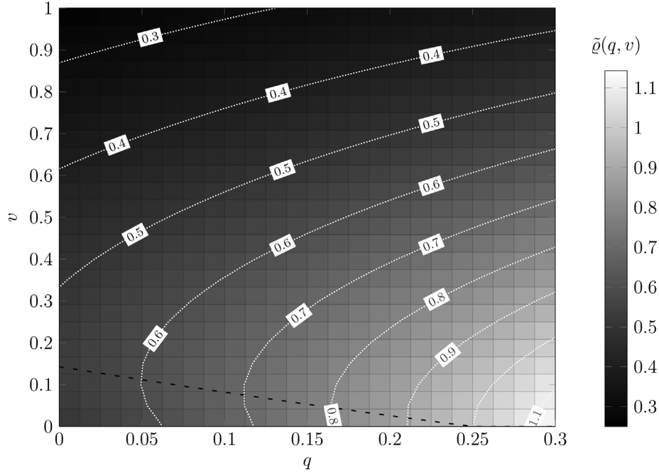
FIGURE 4 Density plot with contours of the \tilde{\varrho} as a function of q and v , \varrho is set to 0.5. The dashed line demarcates two regions, below walk-ins aggravate the variation, conversely above an increase in v reduces the coefficient of variation
