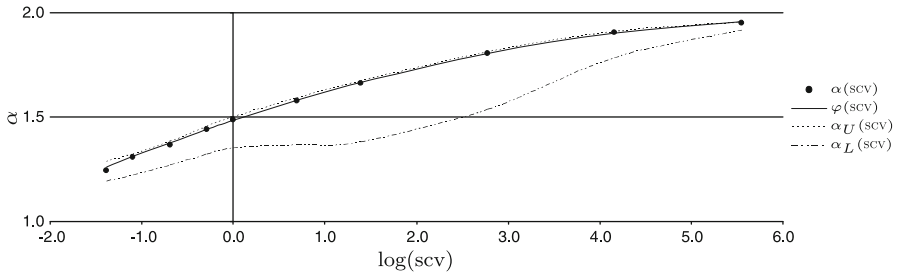
Fig. 2 Graph with BM bounds, simulated values, and approximated values for load \rho = 0.1
